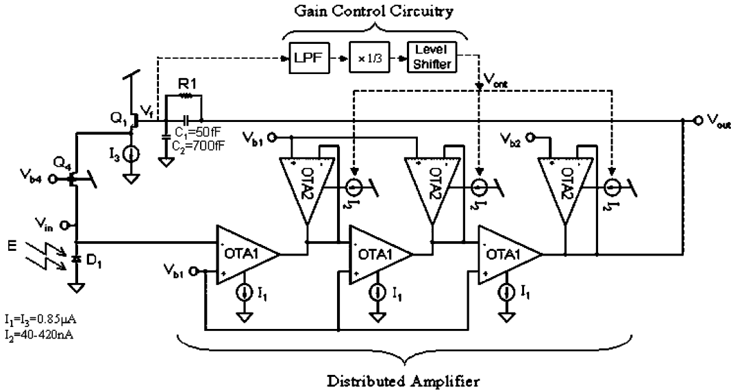
Fig. 4. Circuit schematic of each logarithmic transimpedance amplifier used in our pulse oximeter system of Fig. 1. This circuit employs distributed amplification and automatic loop gain control. (All of the transistors in this figure have W = L = 4.8 \mu\text{m} .)
