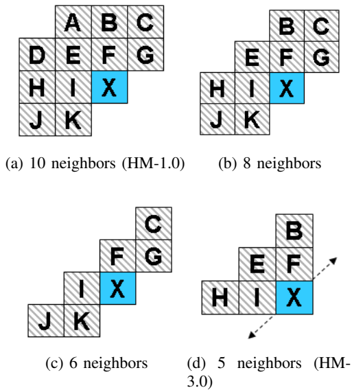
Fig. 2: Neighbor dependencies for SCF context selection. X in blue represents the current position of the bin being processed.
