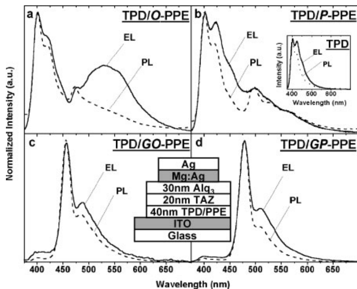
Figure 2. EL spectra (solid line) overlaid with the corresponding PL spectra (dashed line) of the various TPD/PPE LEDs. a,b) Spectra for ungrafted PPE devices (O-PPE and P-PPE, respectively). Inset to (b): plot of the EL and PL of a TPD control device. c,d) Spectra for devices containing grafted PPE (GO-PPE and GP-PPE, respectively). Inset: device structure. The TPD/PPE layer is spin-cast onto clean, indium tin oxide (ITO)-coated glass substrates with a thickness of 50 nm for ungrafted PPE blends and 40 nm for grafted PPE blends. This is followed by thermal evaporation of a 20 nm thick film of TAZ, a 30 nm thick film of Alq 3 , and a 1 mm diameter, 100 nm thick Mg:Ag (10:1 by mass) cathode, with a 30 nm Ag cap. The spin-casting and device manipulation during fabrication is conducted in a dry-nitrogen environment, with moisture and oxygen content of less than 5 ppm. All EL measurements were carried out in air.
