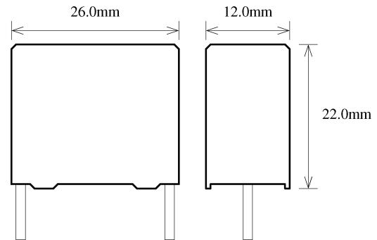
Fig. 22. Dimensioned illustration of Vishay BCcomponents 2222-338-24105 capacitor.
