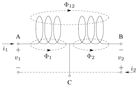
Fig. 3. Flux linkage in “center-tapped” magnetically coupled windings.
