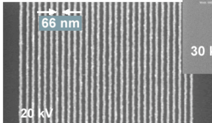
Grating Cr/Si
