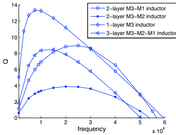
Fig. 4. Quality factor analysis for the four inductors.
