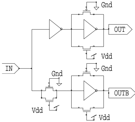
Figure 8: Limited Swing Differential Transmitter
