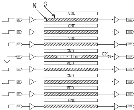
Figure 2: A 8-bit global bus 3000\mu long. Metal line width W = 3\mu , metal line to metal line spacing S = 1.5\mu . A shield line of alternating VSS/VDD connectivity is inserted between alternating signal lines.
