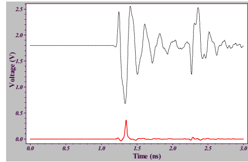
Figure 19: Input and output noise signal to the middle standard receiver buffer in Figure 18. Peak noise on buffer input OP1=1.12V. Peak noise on buffer output OP2=360mV.
