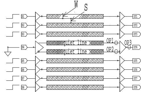
Figure 15: An 8-bit, 3000 \mu long, global bus of 7 standard signals and a differential signal located in the center of the bus. W = 3\mu , S = 1.5\mu . The bus is sandwiched between a VDD line and a VSS line. The driver of the differential signal is a limited swing differential driver and the receiver is a differential receiver. The drivers and receivers of all the standard bits are standard CMOS buffers.
