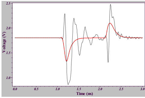
Figure 5: Noise signal measured at OP1 in Figure 1 for a bigger width W = 7.5\mu and S = 1.5\mu . Solid graph represents noise when inductance is NOT modeled (peak noise=0.47V). Dotted graph represents noise when inductance is modeled (peak noise=0.94V).
