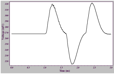
Figure 12: The difference between the signals on points OP1 and OP2 of the differential in Figure 10. This represents the input noise signal to the differential receiver (maximum cross-talk noise is only 53mV).
