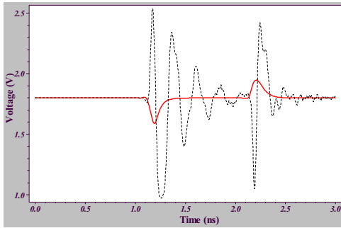
Figure 6: Noise signal measured at OP1 in Figure 1 for a bigger spacing W = 3.0\mu and S = 5.5\mu . Solid graph represents noise when inductance is NOT modeled (peak noise=0.21V). Dotted graph represents noise when inductance is modeled (peak noise=0.82V).
