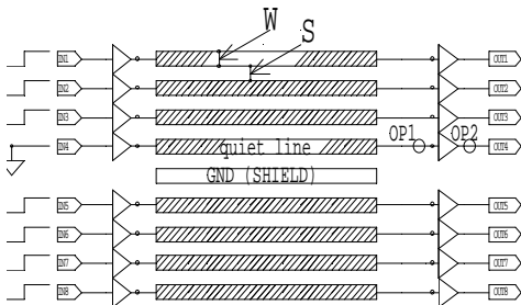
Figure 18: An 8-bit global bus 3000\mu long. W = 3\mu , S = 1.5\mu . A grounded shield wire of width W = 3\mu is inserted in the middle of the bus. The bus is sandwiched between a VDD line and a VSS line. The driver and receiver of each line is a standard CMOS buffer.
