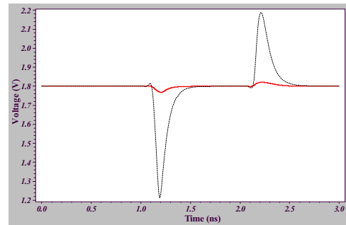
Figure 4: Solid graph represents the noise signal in the shielded example measures at OP1 in Figure 2 (peak noise=0.03V) when the inductance of the interconnect is not modeled. Dotted graph represents the noise signal in the standard single ended example measured at OP1 in Figure 1 (peak noise=0.59V) when the inductance of the interconnect is not modeled.
