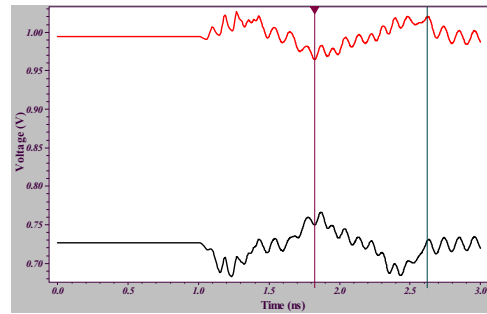
Figure 11: The signal on points OP1 and OP2 of the differential receiver in Figure 10.
