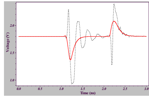
Figure 7: Noise signal measured at OP1 in Figure 1 with each interconnect line in the bus is divided into two 1500\mu segments with a buffer inserted in between the two segments. Solid graph represents noise when inductance is NOT modeled (peak noise= 0.43V). Dotted graph represents noise when inductance is modeled (peak noise=0.87V).
