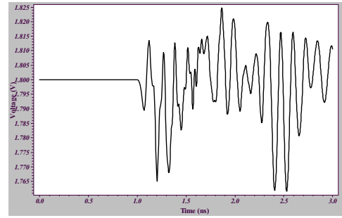
Figure 14: The noise signal on point OP1 in Figure 13. (peak noise is only=38mV).
