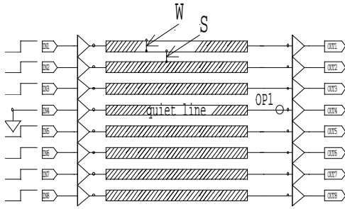
Figure 1: A 8-bit global bus 3000\mu long. Metal line width W = 3\mu , metal line to metal line spacing S = 1.5\mu . The bus is sandwiched between a VDD line and a VSS line each 15\mu wide. The driver and receiver of each line is a standard CMOS buffer.
