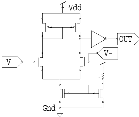
Figure 9: Differential Receiver
