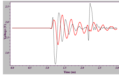
Figure 3: Solid graph represents the noise signal in the shielded example measures at OP1 in Figure 2 (peak noise=0.54V). Dotted graph represents the noise signal in the standard single ended example measured at OP1 in Figure 1 (peak noise=1.17V). Note that the inductance of the interconnect is modeled.
