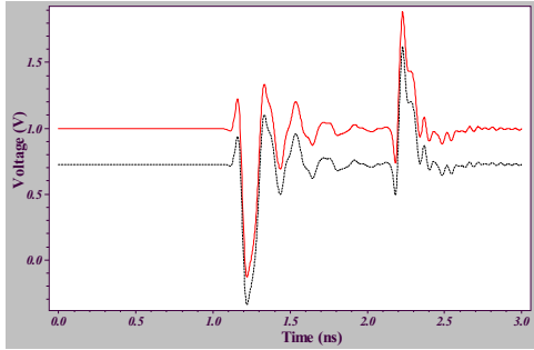
Figure 16: The input signals to the differential receiver, OP1 and OP2 in Figure 15.
