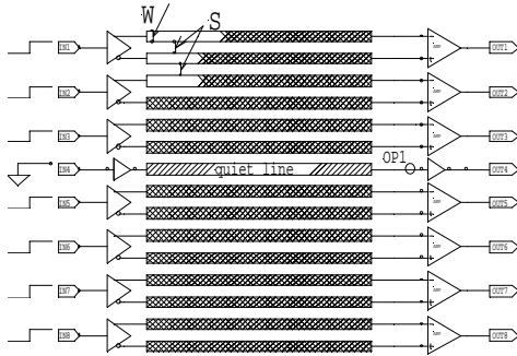
Figure 13: A 8-bit global bus with 7-bits differential (14 signal lines) 3000 \mu long. W = 3\mu , S = 1.5\mu . The non-differential (standard) bit signal is placed in the middle of the differential signals.
