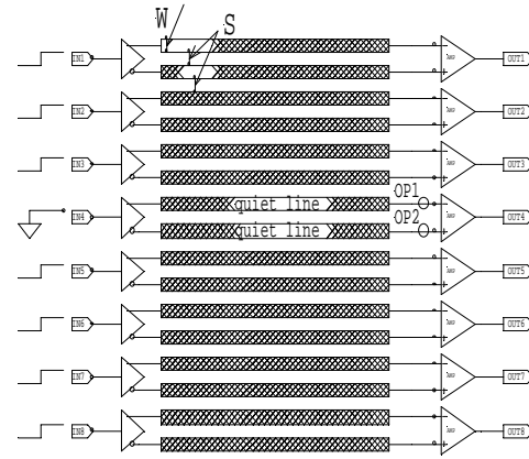
Figure 10: A 3000\mu long global bus with 8-bits differential. The driver of the differential signals is a limited swing differential driver and the receiver is a differential receiver. Metal line width W = 3\mu , metal line to metal line spacing S = 1.5\mu . The 16 line bus is sandwiched between a VDD line and a VSS line each 15\mu wide.
