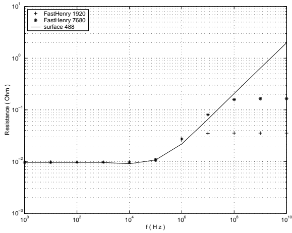
Figure 8: Resistance of a spiral
