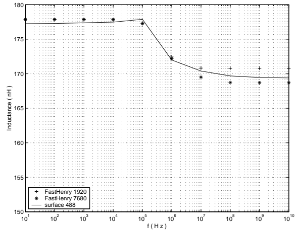
Figure 9: Inductance of a spiral
