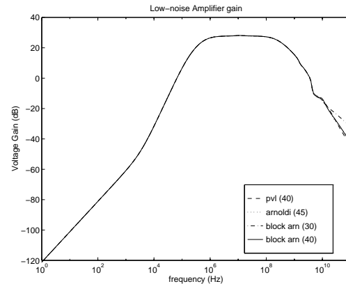
Figure 2: Low-noise amplifier voltage gain approximations. Shown in the figure are the following approximations: 40^{th} order Padé, 45^{th} order Arnoldi, 30^{th} and 40^{th} order block Arnoldi. The 40^{th} order block Arnoldi results are indistinguishable from the exact gain.
