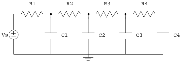
Figure 1: RC-circuit that shows that the Lanczos algorithm can produce an unstable model even if the system is described by a symmetric positive definite matrix.
