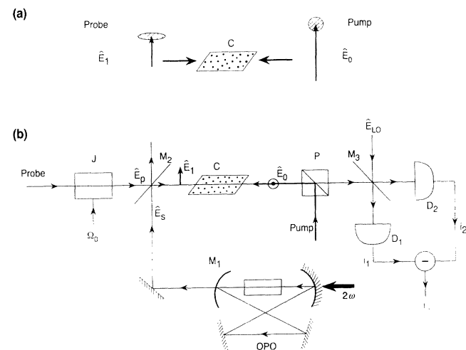
FIG. 1. (a) Saturation spectroscopy with squeezed light. The sample cell C is illuminated by the squeezed probe \hat{E}_1 and by a coherent pump \hat{E}_0 , with the error circle for \hat{E}_0 representing vacuum-state fluctuations and the error ellipse for \hat{E}_1 indicating fluctuations for a squeezed state. (b) Experimental setup for FM spectroscopy with squeezed light.
