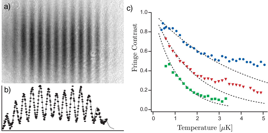
Figure 5-3: High contrast interference of a thermal cloud of atoms. a) Absorption image taken after 48 ms expansion. b) The integrated optical density is fit to Equation 5.4, resulting in a value for the fringe contrast C . c) Measured fringe contrast C as a function of temperature, for fringe spacing \lambda_F = 340 \mu\text{m}, 230 \mu\text{m}, 170 \mu\text{m} (circles, triangles, squares). The theoretical contrast of Equation 5.8 (dashed lines) describes the data well at low temperature.
