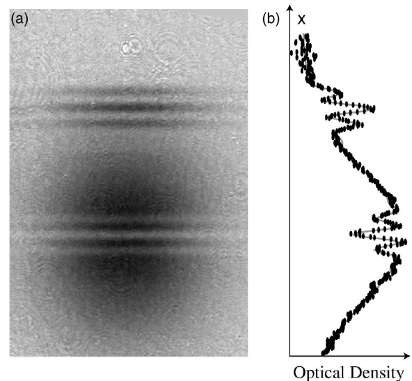
FIG. 4. Velocity-selective Bragg diffraction: (a) Absorption image of atoms subject to 40- \mu s Bragg pulses. The fringe spacing was \lambda_f=210 \mu m after 48 ms time of flight. These longer Bragg pulses addressed only a subset of the momentum distribution. (b) Cross section and fit (black circles and gray line, respectively).
