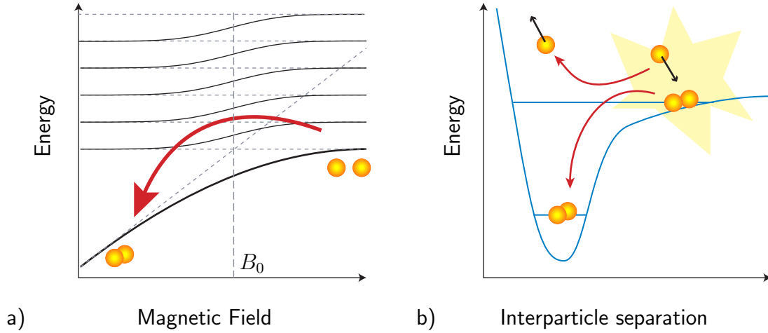
Figure 2-4: Feshbach Molecules. a) The atom-molecule coupling near a Feshbach resonance creates an avoided crossing between the free atom continuum and a bound molecular state. Atoms can be adiabatically converted to molecules by sweeping the magnetic field across the resonance. b) Three body collisions can transfer weakly bound molecules into a more deeply bound state, while a third body carries off the difference in binding energy as kinetic energy.
