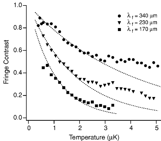
FIG. 3. Contrast vs temperature for 10- \mu s Bragg pulses. Different fringe spacings \lambda_f were realized by varying the wait time \tau_w between the two Bragg pulses. The time of flight was kept fixed at 48 ms. At lower temperatures the observed contrast agreed well with theory (dashed lines) given by Eq. (3). At higher temperature, however, the contrast was higher than predicted, owing to the velocity selectivity of the Bragg pulses. The BEC transition temperature was at T_c=0.6 \mu K.
