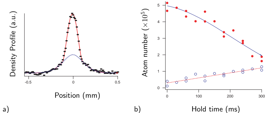
Figure 7-4: Dissipation in a moving lattice. a) A bimodal fit of the density profile, after 17 ms expansion, provides a measure of the heating incurred in the moving lattice. b) The number of pairs in the thermal component N_{th} (open circles) and those remaining in the condensate N_c (filled circles) as a function of the time held in the moving lattice. The thermal component grows approximately linearly (dashed line), whereas N_c is fit to model (solid line) in which the loss is proportional to N_{th} (Equation 7.18).
