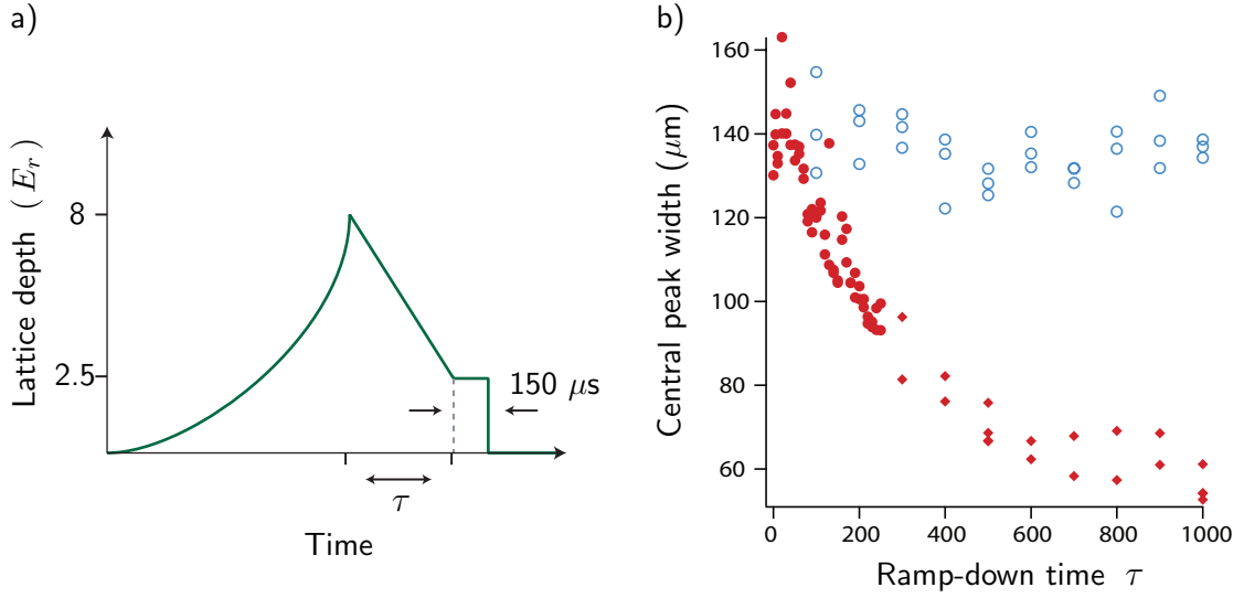
Figure 6-5: Restoring coherence from a deep lattice. a) The lattice is adiabatically ramped up to V_0 = 8 E_r . A sample released from a lattice of this depth does not exhibit interference. In order to study the time scale on which coherence can be reestablished, we ramp V_0 down to 2.5 E_r over a variable ramp time \tau . The sample is held here for 150 \mu\text{s} , while the magnetic field is ramped down, before release. b) As a measure of coherence, the widths of the central peak after 6.5 \text{ ms} expansion, obtained from a gaussian (bimodal) fit, are plotted as solid circles (diamonds), as a function of \tau . The fast time scale over which coherence is restored indicates that the sample stays in the ground state during the application of the lattice. A sample which has been decohered (open circles), through the application of a magnetic gradient during the lattice ramp-up, does not regain coherence under the same conditions.
