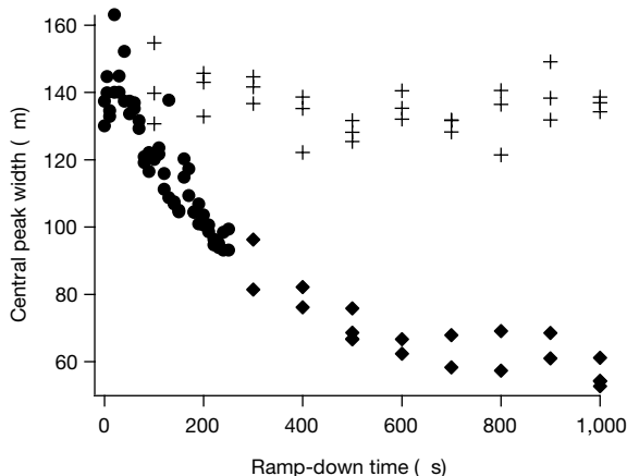
Figure 5 | Restoring coherence from a deep lattice. The width of the central peak is used as a measure of phase coherence after an adiabatic ramp up to 8E_F , followed by a fast ramp down to 2.5E_F at a fixed magnetic field of 822 G. Filled circles were extracted with the use of a gaussian fit, and diamonds with a bimodal fit. Also plotted for comparison is the gaussian width of the central peak for a dephased sample, in which a field gradient was applied during the ramp up of the lattice (crosses). All points were taken for 6.5 ms time of flight.
