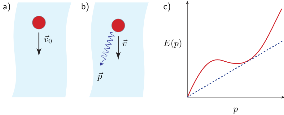
Figure 7-1: The Landau criterion for superfluidity. (a) An object passing through a fluid with velocity v_0 can (b) create an excitation in the fluid with momentum p . As a result, the motion is damped, reducing the velocity to v . Conservation of energy and momentum place a lower bound on the velocity for which excitations can occur, known as the Landau criterion (Equation 7.4). (c) This critical velocity, v_c = \min E(p)/p , can be depicted graphically as the slope of a (dashed) line which is tangent to the dispersion relation E(p) (solid line).
