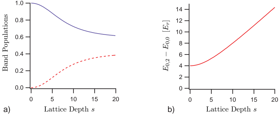
Figure 4-5: Band populations and energy gap. a) At a lattice depth s , the zero momentum state is a superposition of the eigenstates with zero quasimomentum in the n = 0 and n = 2 bands. The weightings of \psi_{0,0} (solid line) and \psi_{0,2} (dashed line) are shown (see also Equation 4.3). b) The energy difference between the n = 0 and n = 2 bands at Q = 0 sets the oscillation frequency of Kapitza-Dirac scattering, and can be approximated by Equation 4.4.
