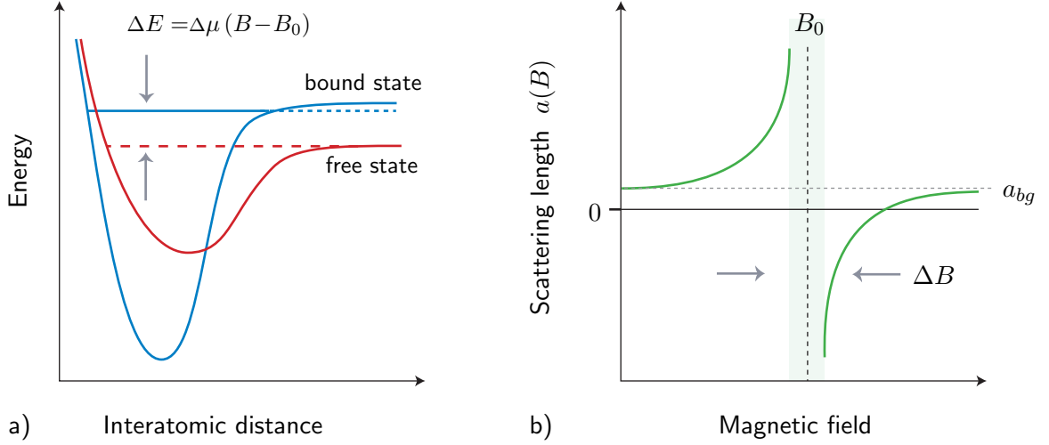
Figure 2-3: The Feshbach resonance. a) Interatomic potentials for different spin configurations have a difference in magnetic moment \Delta\mu , and thus tune differently with magnetic field. A free atomic state (red line) becomes degenerate with a bound molecular state (blue line) at a magnetic field B_0 . b) Due to a coupling between these two states, two-body scattering is resonantly enhanced near this field. The s-wave scattering length a diverges on resonance, and can be tuned in both magnitude and sign in the region \Delta B around resonance. The general form for a(B) is found in Equation 2.12.
