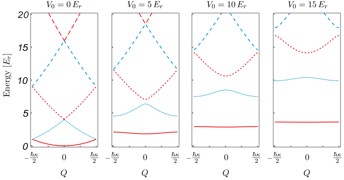
Figure 3-6: Band structure. A lattice potential modifies the free particle dispersion relation. The translational symmetry allows us to describe a state by its quasi-momentum Q and band index n . In the limit of large lattice depth, the bands flatten and become the harmonic oscillator energies for atoms on a single lattice site.
