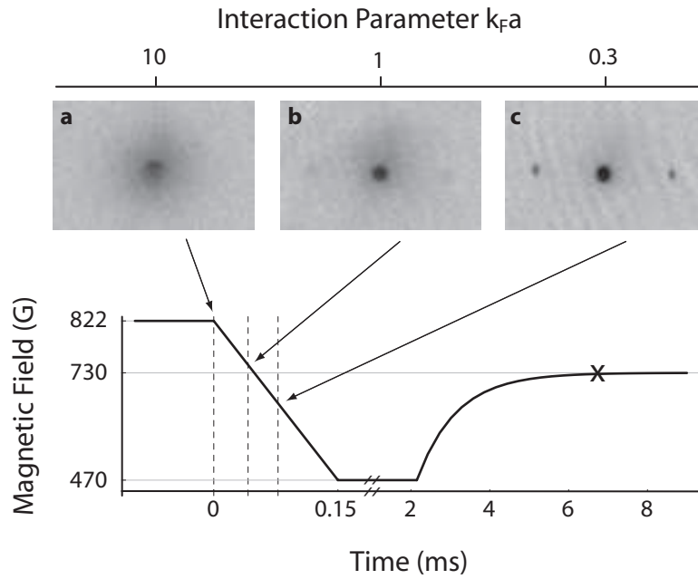
Figure 6-1: Dissipative collisions between momentum components. A Li pair condensate is prepared at 822 G. The magnetic field is cut abruptly when the cloud is released from the trap. As a probe of the scattering cross section \sigma , a short Kapitza-Dirac pulse is administered at different times during the field ramp, corresponding to magnetic fields (a) 822 G, (b) 749 G and (c) 665 G. The absorption images reveal different degrees of heating due to collisions between the discrete momentum components. For a sufficient reduction of the interaction parameter k_F a , and therefore the scattering cross section, the distinct momentum peaks are visible.
