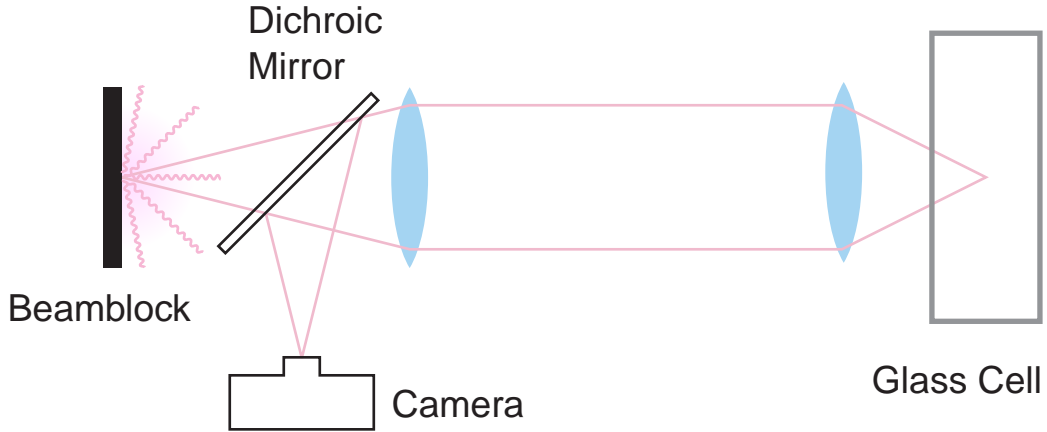
Figure 4-4: An accidental lattice. An optical dipole trap (ODT) is aligned on the imaging axis. A long wave pass dichroic transmits the ODT beam, which impinges on a beamblock. When the beamblock is located at the focus of the imaging system, much of the scattered light is imaged back onto the atomic sample, interfering with the incident ODT beam to produce a lattice.
