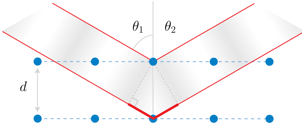
Figure 3-5: X-ray diffraction. The angle of diffraction of a wave off a lattice of point scatterers is given by the Bragg condition, Equation 3.21. This describes the condition for constructive interference of the various scattered components.
