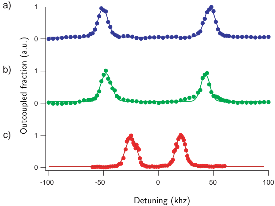
Figure 3-8: Bragg spectroscopy of atoms and molecules. The spectra for a pure atomic sample a) just above and b) below a magnetic Feshbach resonance at 907 G. c) Spectrum of a pure molecular sample just below the Feshbach resonance. Diatomic molecules recoil with half the velocity of single atoms, due to their mass. Figure from [1].
