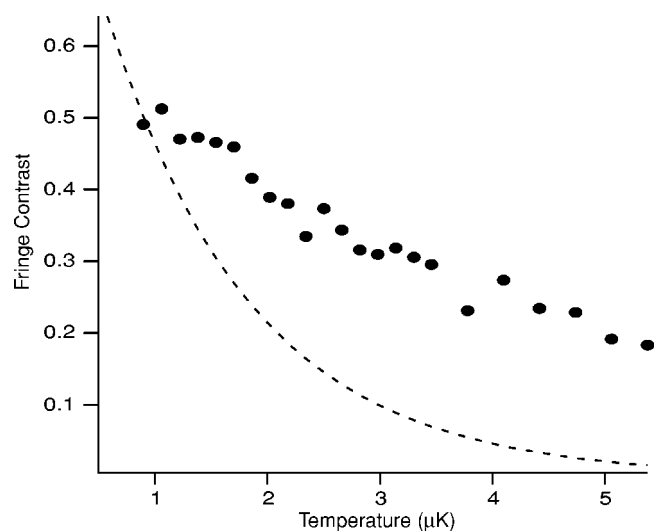
FIG. 5. Measured contrast for \tau_p=30 \mu s velocity-selective Bragg pulses. The contrast was significantly higher than that predicted by Eq. (3) (dashed line). The fringe spacing was \lambda_f=170 \mu m after 48 ms expansion time.
