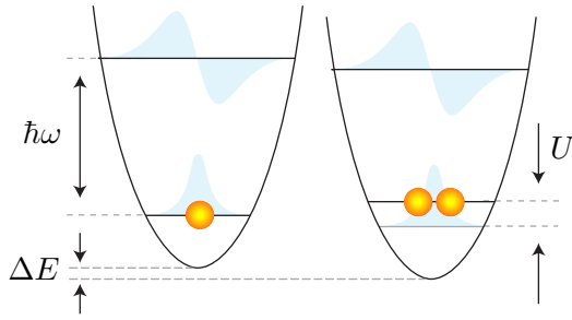
Figure 6-3: Individual lattice sites can be approximated as harmonic oscillators with energy spacing \hbar\omega . For repulsive interactions, there is an energy cost U for two atoms to occupy the same lattice site. The application of a potential gradient results in an energy difference \Delta E between sites. For a conducting state, this will result in current. An insulating state, however, will not respond.
