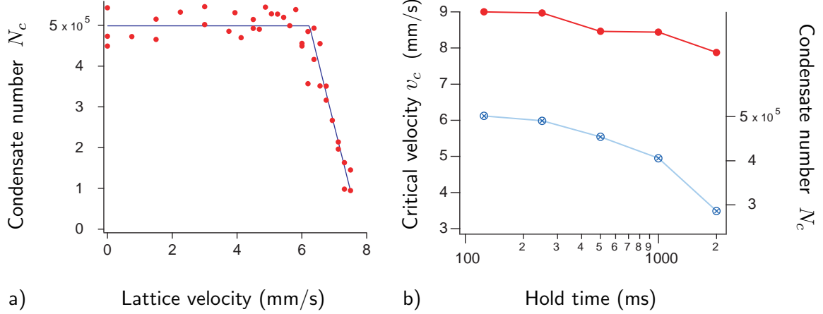
Figure 7-6: Critical velocity at the cloud center. a) Number of pairs which remained in the condensate N_c after being subjected to a V_0 = 0.2 E_F deep optical lattice for 500 ms, moving with velocity v_L , at a magnetic field of 822 G ( 1/k_F a = 0.15 ). An abrupt onset of dissipation is observed above a critical velocity v_c , which we identify from a fit to Equation 7.19. b) The critical velocity we obtain (filled circles) is weakly dependent on the time held in the lattice (logarithmic scale). Some of this variation may in fact be attributed to the reduction in numbers, and therefore speed of sound, due to the sample’s finite lifetime. We show N_c as a function of hold time in a stationary lattice (crossed circles).
