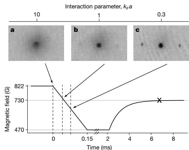
Figure 1 | Dissipative collisions during expansion of a strongly interacting fermionic superfluid. The schematic shows the time sequence of the magnetic field ramp used throughout this paper. A one-dimensional optical standing wave was pulsed onto the superfluid at different magnetic fields B_p (indicated by arrows at 822 G (a), 749 G (b) and 665 G (c)) during expansion, creating particles at twice the photon recoil 30 . Absorption images taken at the time marked with the cross show distinct momentum peaks only at magnetic fields B_p \leq 750 G, where k_F a \leq 1 . At higher magnetic fields, the peaks blurred into a broad diffuse cloud as a result of the larger collision cross-section.
