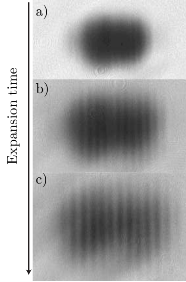
Figure 5-5: Contrast emerges in time of flight. The coherence length \ell_c grows during expansion, and eventually exceeds the initial separation d = 2 \mu\text{m} . Expansion time is a) 14 ms, b) 20 ms, and c) 25.
