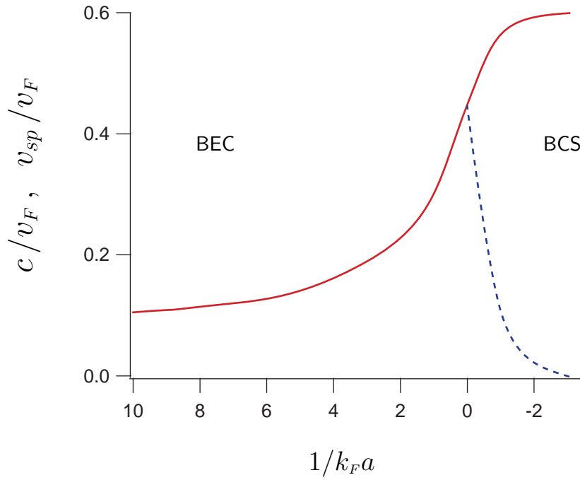
Figure 7-2: Speed of sound and pair-breaking threshold in a two-component Fermi gas. The speed of sound c (solid line) increases monotonically across the BEC-BCS crossover. The threshold velocity v_{sp} for pair-breaking falls exponentially in the BCS limit. The Landau critical velocity is given by the minimum velocity of these two, and is sharply peaked near resonance. Adapted from [26].
