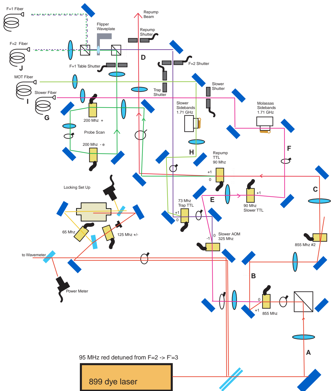
Figure 4-1: The sodium laser table. Letters denote the positions of power measurements as listed in Table 4.1.
