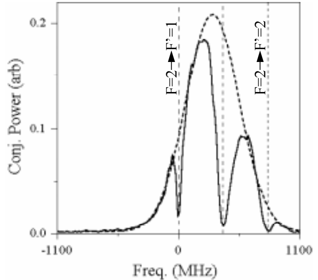
Figure 3. The conjugate power as a function of the laser frequency. The vertical dotted line on the left (right) corresponds to the 5^2S_{1/2} F = 2 to 5^2P_{1/2} F = 1 ( 5^2S_{1/2} F = 2 to 5^2P_{1/2} F = 2 ) transition of the D_1 manifold in ^{87}\text{Rb} .
