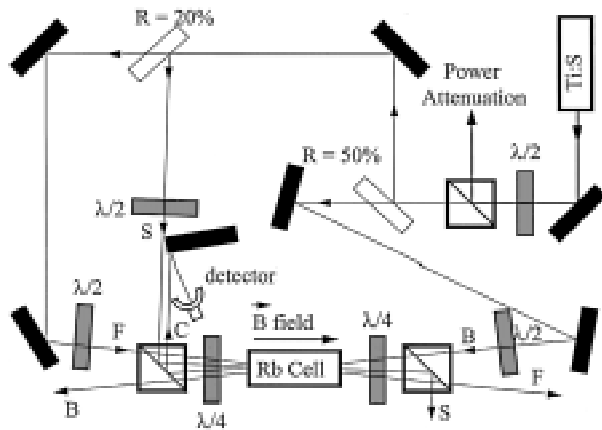
Figure 2. Schematic illustration of the experimental setup. The rubidium cell is a heat-pipe oven, and the pump is a Ti:Sapphire laser. \lambda/2 is a half-wave plate, and \lambda/4 is a quarter-wave plate.
