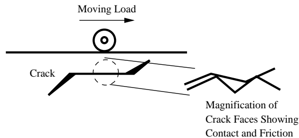
Figure 18. Rolling fretting fatigue causing nonlinear mechanical behavior through contact and friction.
