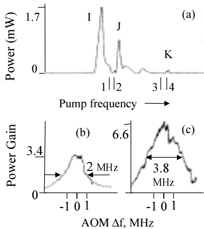
Figure 10. (a) PCR intracavity power as a function of the pump frequency. The numbers 1 through 4 correspond to the following D_1 transitions: (1) F = 2 \leftrightarrow F' = 1 (2) F = 2 \leftrightarrow F' = 2 (3) F = 1 \leftrightarrow F' = 1 , and (4) F = 1 \leftrightarrow F' = 2 . (b) The PCM conjugate gain as a function of \Delta f for the two pump intensities (1) 4.6 \text{ W/cm}^2 and (2) 10 \text{ W/cm}^2 .
