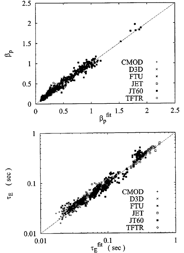
Figure 21. Comparison of the \beta_p and \tau_E scalings with experimental data.
