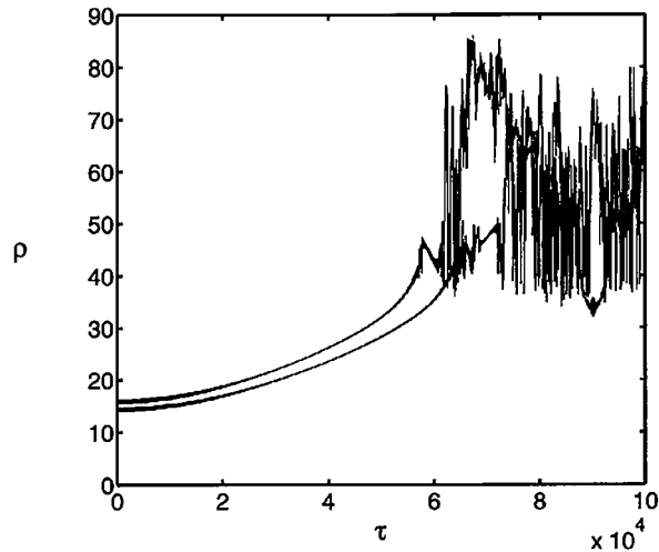
Figure 9. Normalized Larmor radius \rho versus \tau for two ions interacting with two waves. The parameters are the same as in Figure 8 except that \kappa = 1.02 , i.e., the higher frequency wave has the shorter wavelength.
