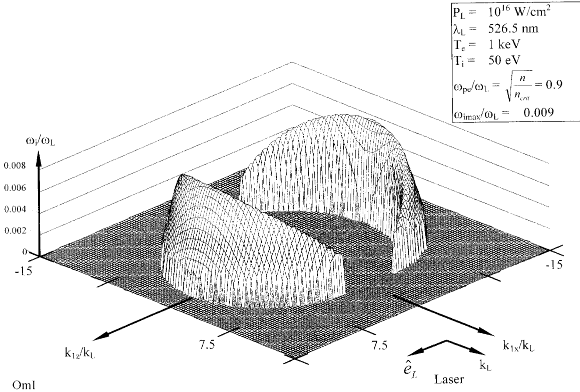
Figure 16. Normalized growthrate, \omega_r(k_r)/\omega_L , for the PP interaction plotted in the k_{1x} - k_{1z} plane.
