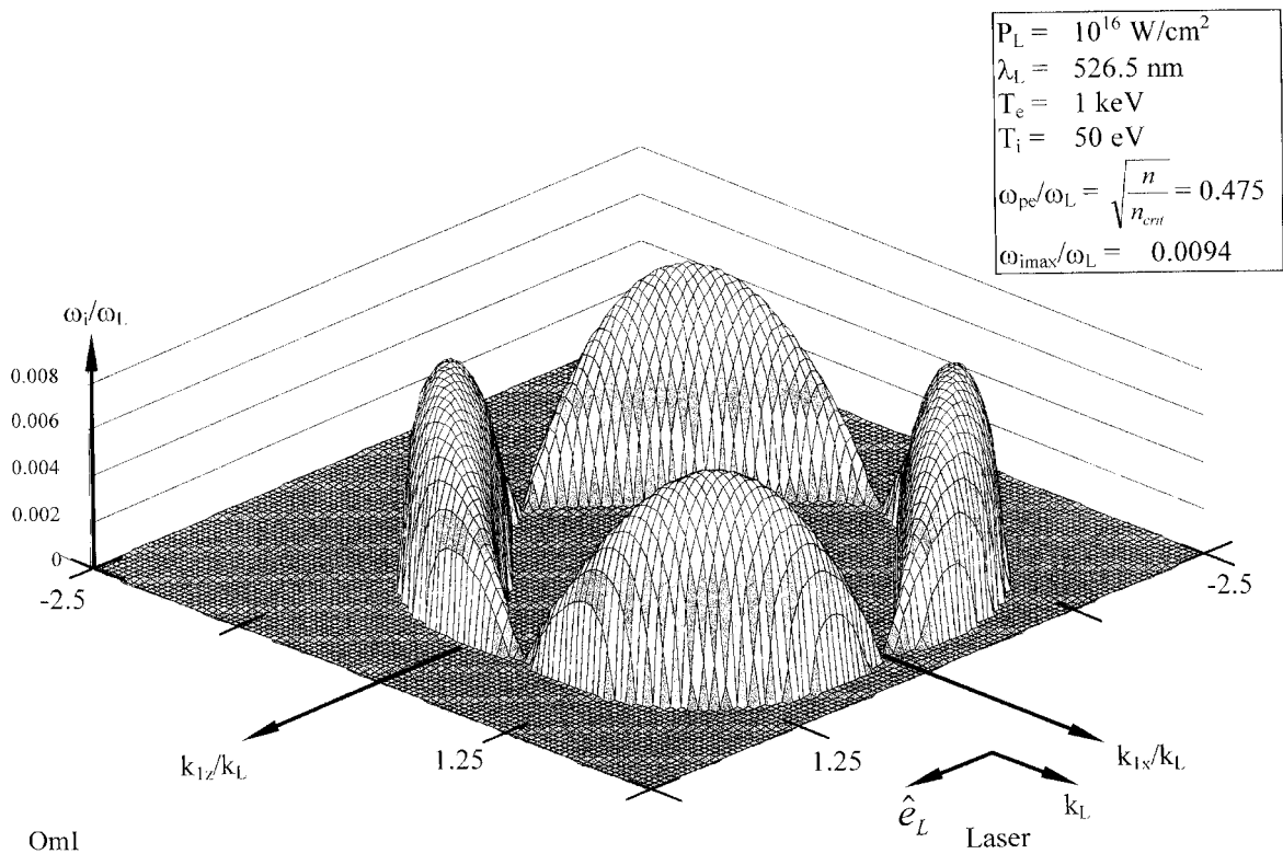
Figure 15. Normalized growthrate, \omega_i(k_r)/\omega_L , for the TP interaction plotted in the k_{1x} - k_{1z} plane.
