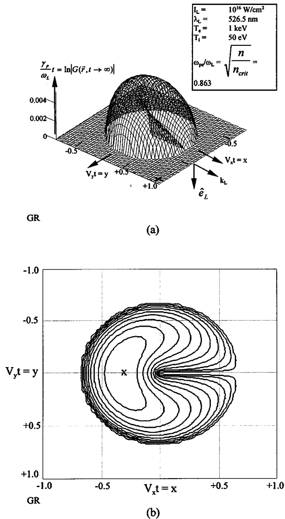
Figure 19. (a) Pulse shape and (b) contour plot for the SBS pinch point growthrate plotted in the V_x - V_y plane. Note that numerical values in x and y are to be multiplied by ct and amplitudes on vertical axis by t . In (b), the outermost contour is zero, the maximum is marked with an "x," and each contour represents a 10% change.
