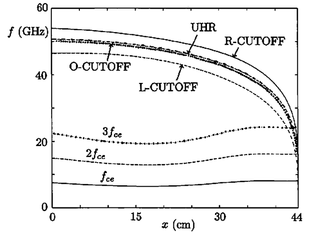
Figure 1. Distribution of critical frequencies in propagation across the magnetic field along the equatorial plane in NSTX (Figure 3). 8
