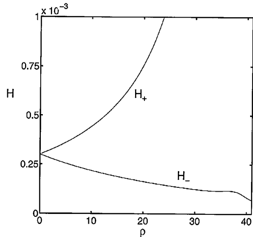
Figure 11. Plot of H_- and H_+ as a function of \rho for parameters corresponding to Figure 9.
