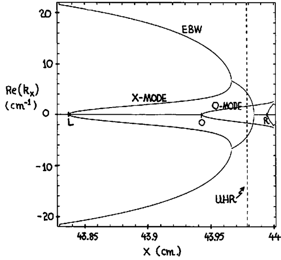
Figure 2. Local kinetic dispersion relation for the same parameters as in Figure 1.
