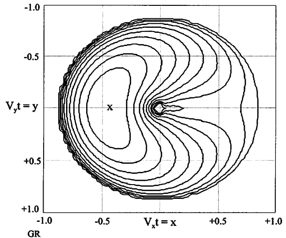
Figure 18. (a) Pulse shape and (b) contour plot for the SRS pinch point growthrate plotted in the V_x - V_y plane. Note that numerical values in x and y are to be multiplied by ct and amplitudes on vertical axis by t . In (b), the outermost contour is zero, the maximum is marked with an "x," and each contour represents a 10% change.
