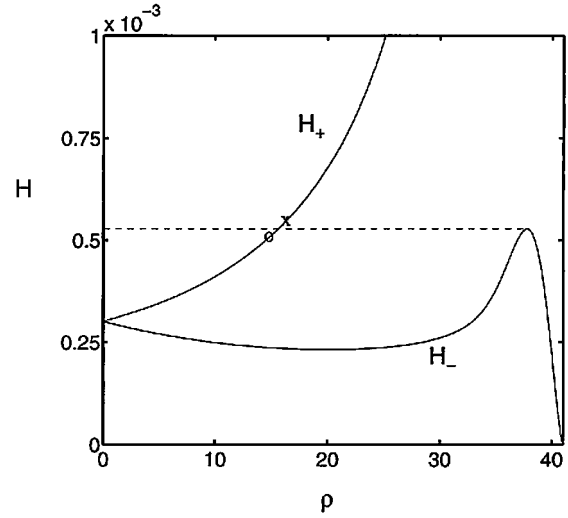
Figure 10. Plot of H_- and H_+ as a function of \rho for parameters corresponding to Figure 8. The dashed line gives the minimum value of H needed to make it into the chaotic region. The circle and the cross mark the initial locations of the two ions of Figure 8.
