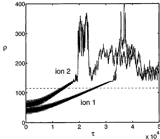
Figure 6. The dynamics of two ions in 162 waves. All the waves have the same normalized wavenumber k_i = 1 and normalized amplitude \epsilon_i = 10.7 , for i = 1, 2, \dots, 162 . The frequencies of these waves are \nu_{3n-2} = 146.2+n , \nu_{3n-1} = 146.381+n , \nu_{3n} = 146.873+n , for n = 1, 2, \dots, 54 . The wavelength and the electric field amplitude of each wave are 2 m and 25 mV/m, respectively. Initially ion 1 has \rho_0^{(1)} = 54 , corresponding to an energy of 2.3 eV, and ion 2 has \rho_0^{(2)} = 76.5 , corresponding to an energy of 4.6 eV. Both ions start off with an initial phase \psi_0 = 0 .
