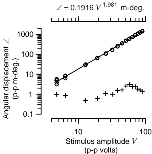
Figure 3. Calibration of fatigue test structure developed by Failure Analysis Associates, Inc. The device used in Figure 2 was stimulated at resonance with a sinusoidal voltage. Five independent measurements (circles) were made at each of 15 different amplitudes (abscissa) of stimulation. The line given by the equation at the top of the plot is a regression line fit by a least squares method. Pluses indicate the standard deviations of results at each amplitude.
