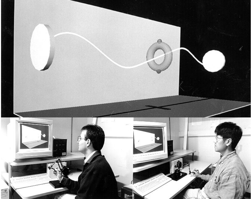
Fig. 2. Our current VR set-up that enables two people, at remote locations, to interact with each other through visual and haptic displays. For example, subjects will be able to hold and move a ring on a wire in a collaborative manner as depicted in this figure. To eliminate time delays due to network connections, we bifurcated the signals from a single host and displayed on two separate monitors. To maintain stable force interactions, the haptic update rate was fixed at 1KHz.
