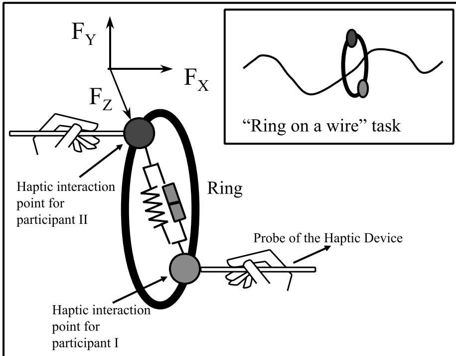
Fig. 5. The proposed model for simulating haptic interactions between participants in SVEs to perform a collaborative task of moving a ring on a wire.
