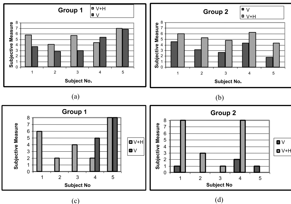
Fig. 6. Subjective scores (i.e., score for “sense of togetherness”) of each subject in groups 1 and 2 are represented as bar charts for comparison of experimental conditions (“V” vs. condition “V + H”). In charts (a) and (b), the subjective measure is based on the average of subjects’ responses to the 8 “togetherness” questions. In charts (c) and (d), the subjective measure is based on the number of “high” (“6” or “7”) responses out of the 8 “togetherness” questions. Results show that subjective sense of togetherness increases with the addition of haptic feedback.
